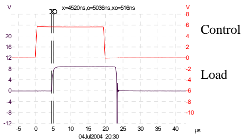
Figure 3 Rising Time is 0.516µS
