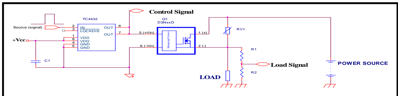
Figure 10 A high-speed Solid State Relay is controlled by a dedicated MOSFET driver.
